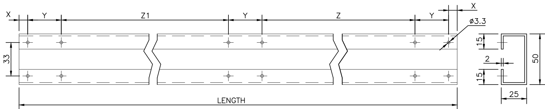
C CHANNEL CROSS SECTION
