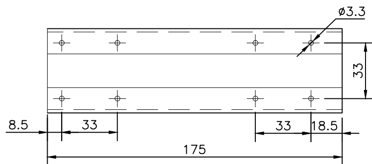
C CHANNEL LENGTH 175
