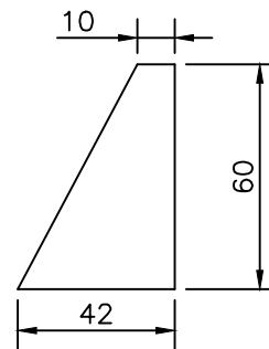
GUSSET
