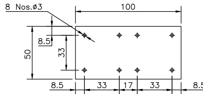
SUPPORT PLATE
