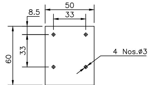
VERTICAL PLATE
