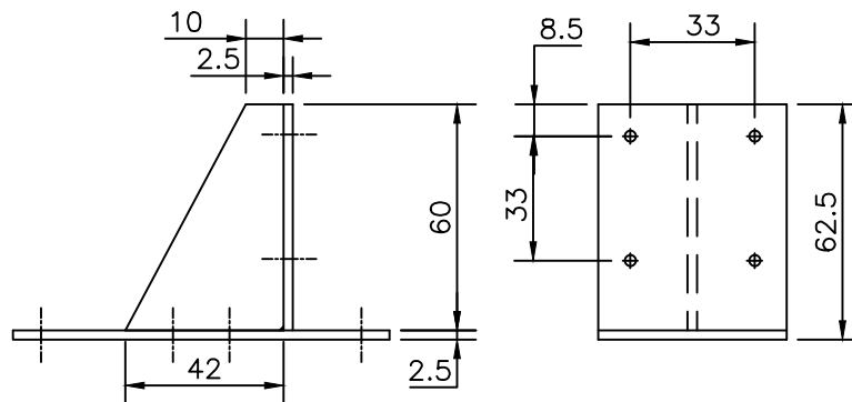
ASSY OF SUPPORT PLATE & GUSSET
